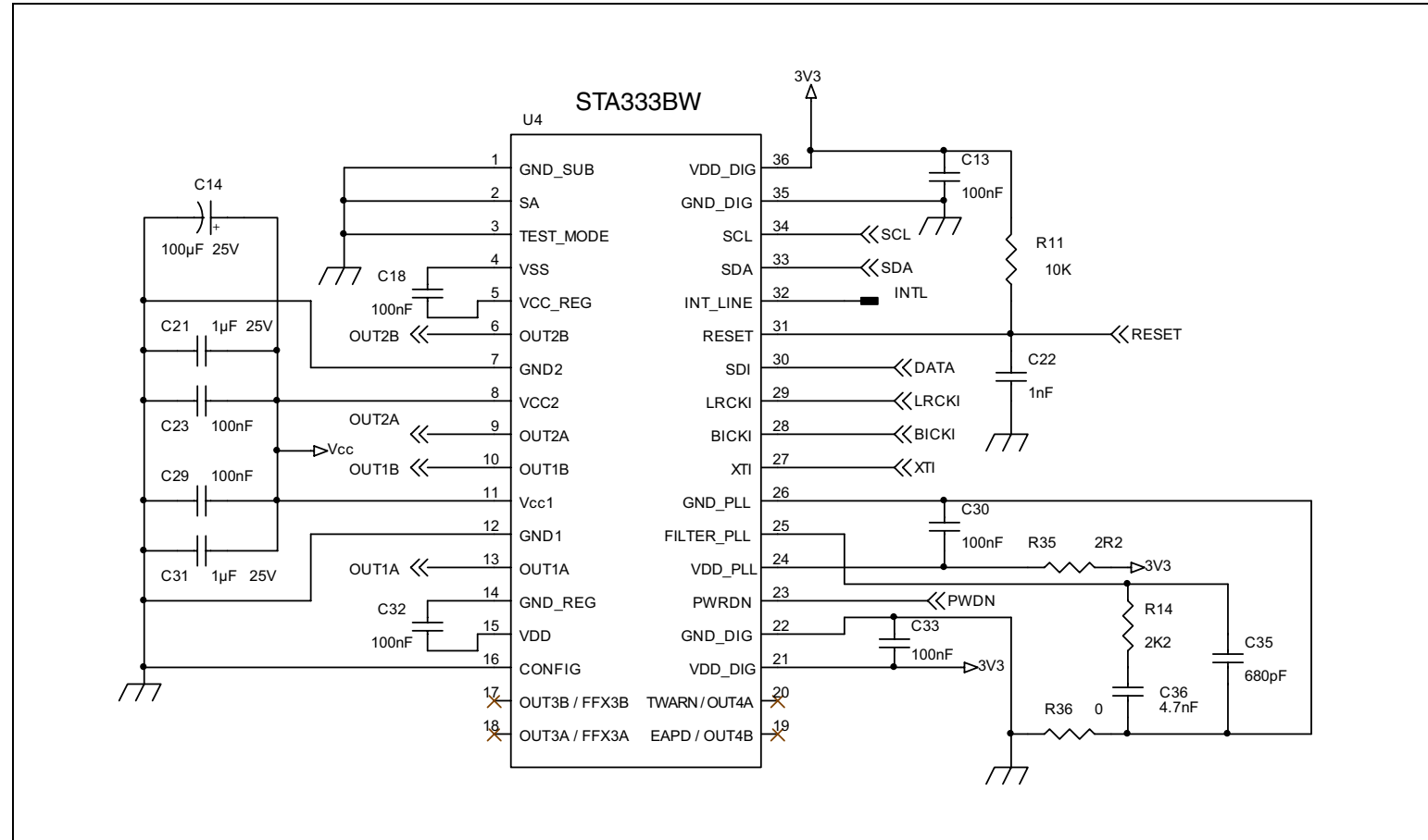
Figure 20. Applications circuit
