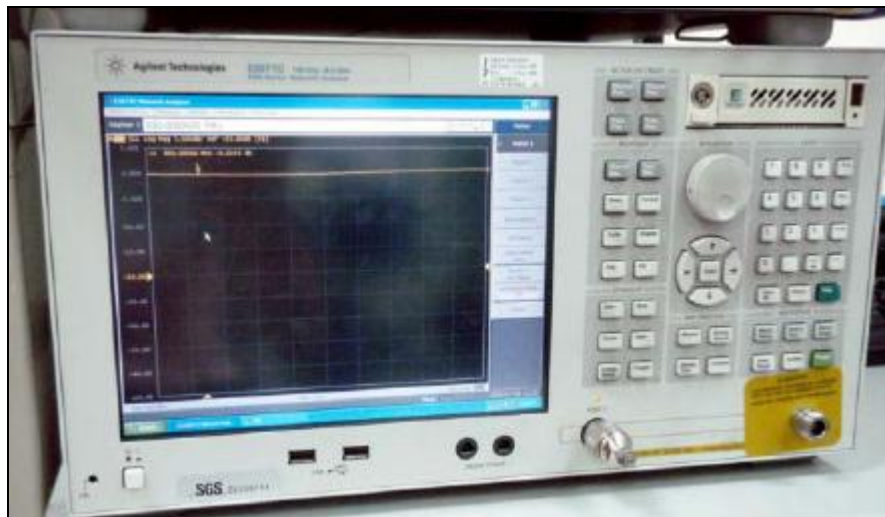
Figure 2. Network Analyzer.
