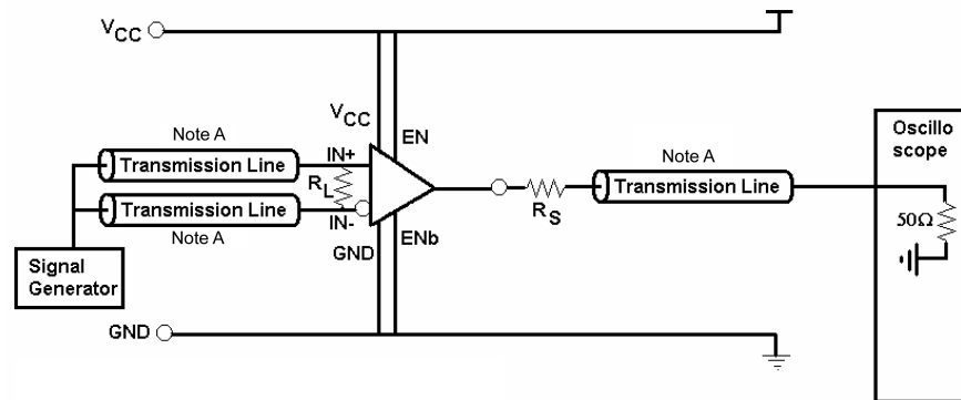
FIGURE 7. LVTTL Output Propagation Delay and Transition Time Test Circuit
