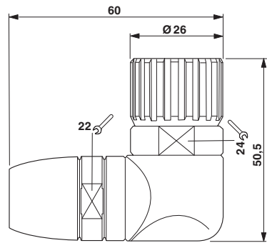
Dimensional drawing
