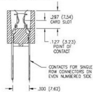
SECTION THROUGH CONTACT POSITION
