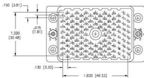
120 PIN PLUG
