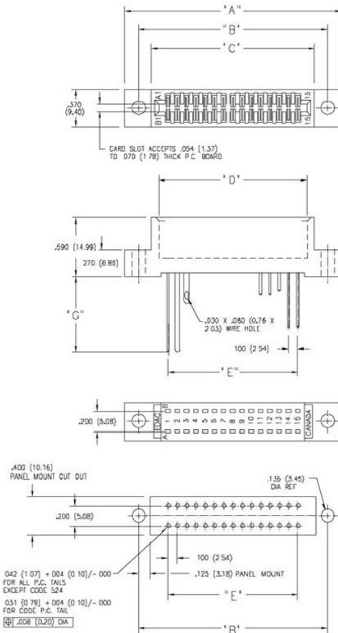
CONNECTOR MOUNTING PATTERN
