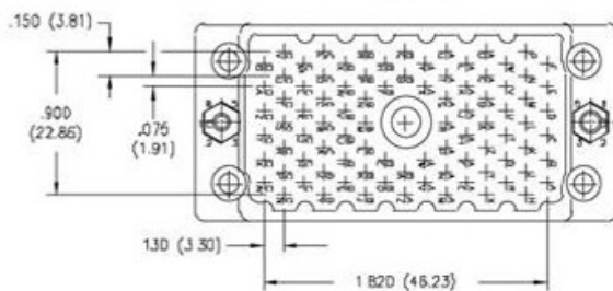
90 PIN PLUG
