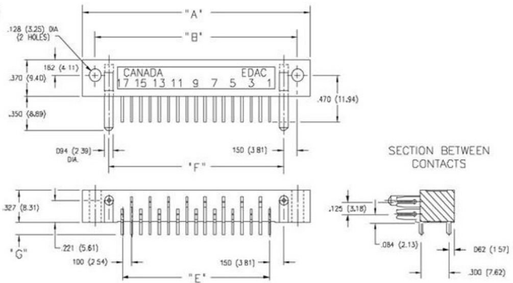
423 SERIES CONNECTOR
