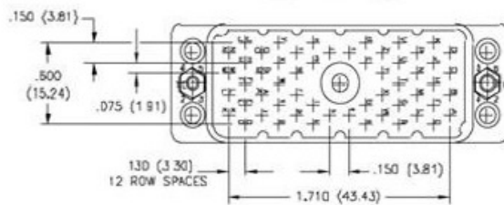
56 PIN PLUG
