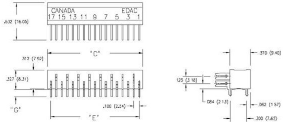
422 SERIES CONNECTOR
