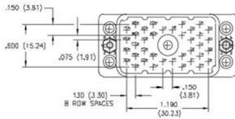
38 PIN PLUG
