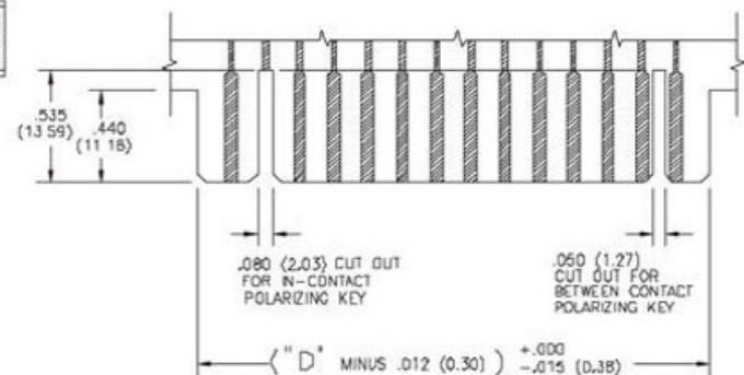
RECOMMENDED DAUGHTER BOARD
