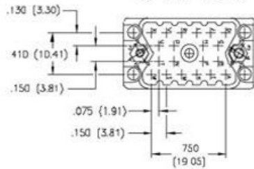
20 PIN PLUG
