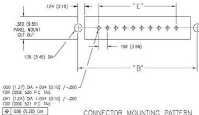
CONNECTOR MOUNTING PATTERN
