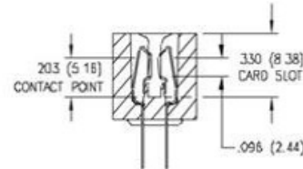
SECTION THROUGH CONTACT POSITION
