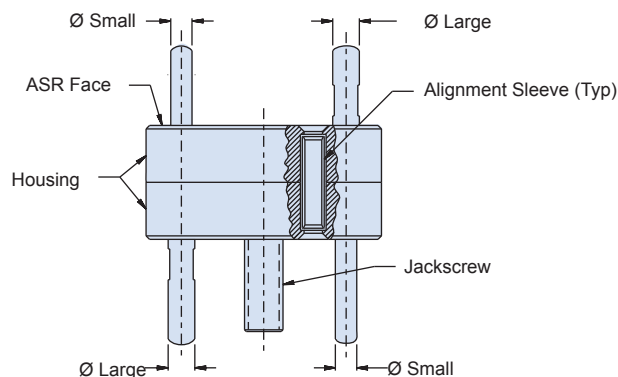
Shell Size 15 Arrangement 10 Shown
