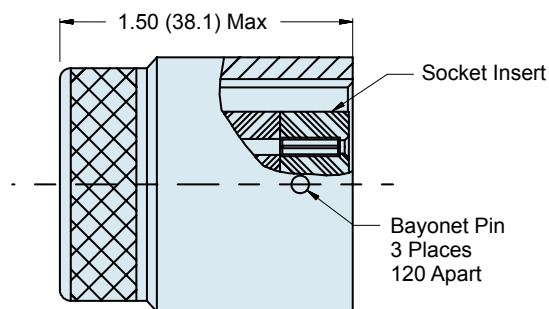
07 Receptacle Adapter U.S. PATENT NO. 5,960,137
