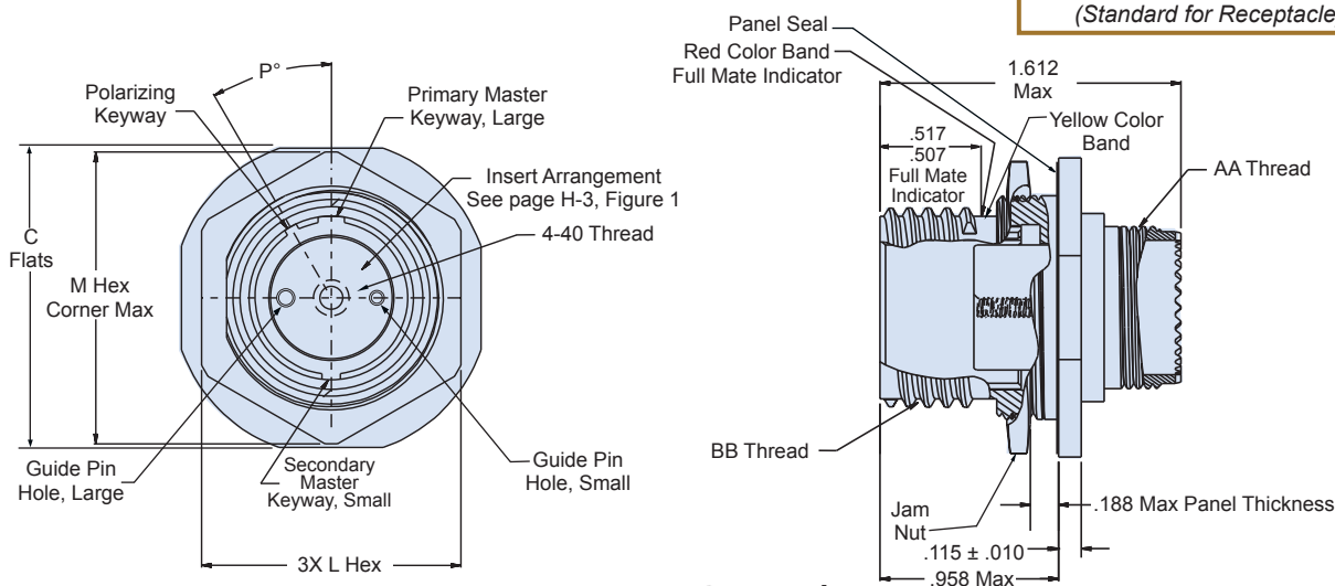
08 - Jam Nut Mount Receptacle
