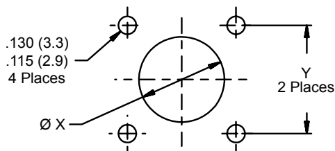
Recommended Panel Cutout (Wall Mounting)
