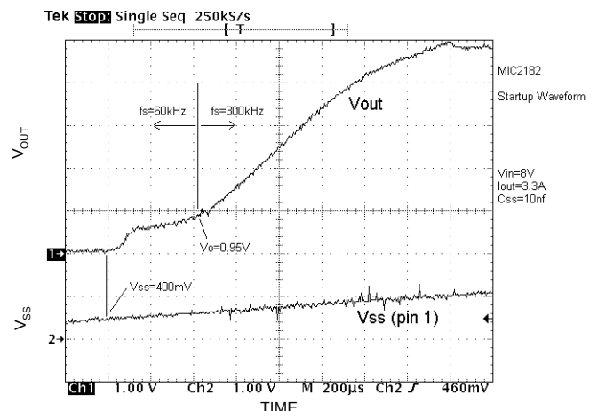
Figure 9. Startup Waveforms
