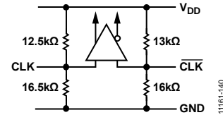
Figure 43. AD9508 Differential Input Stage
