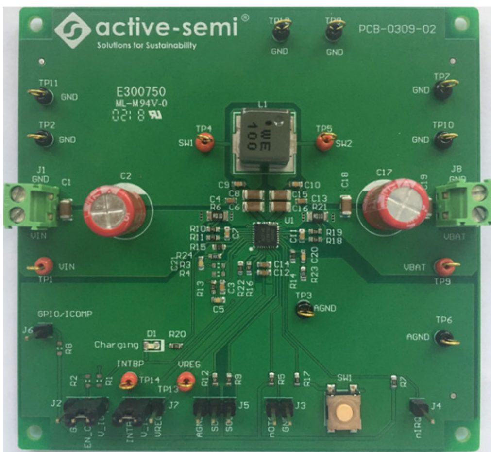
Figure 1 – EVK Picture
