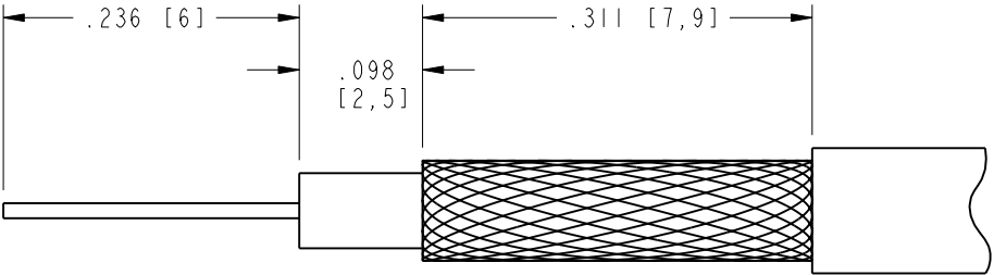
SCALE 6.000 RECOMMENDED CABLE STRIPPING DIMENSIONS
