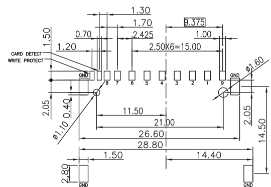
RECOMMENDED P.C.B LAYOUT TOLERANCES: ±0.05mm
