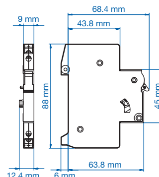
Dimensions HLS11M.
