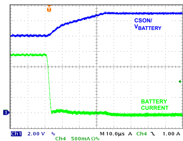
FIGURE 11. BATTERY REMOVAL
