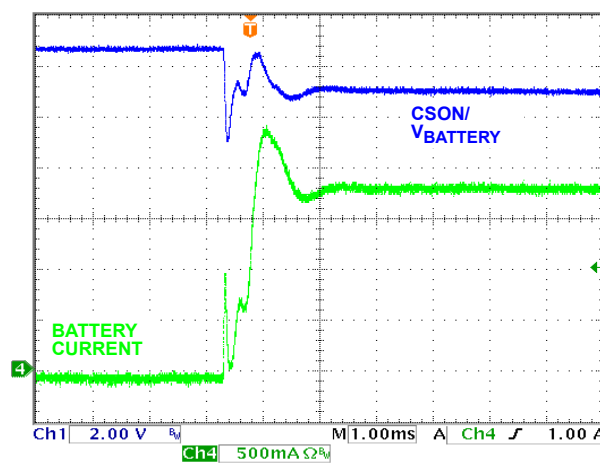
FIGURE 12. BATTERY INSERTION
