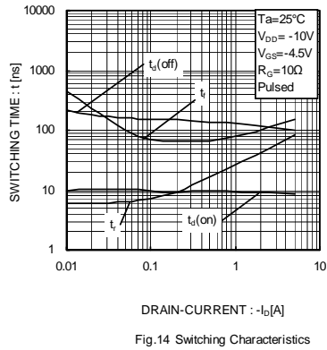
Fig.14 Switching Characteristics
