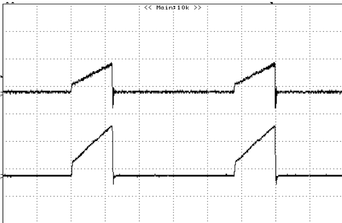
Figure 25: Typical transient response to step load change at 5A/\mu S from 25% to 75% of I_{o, max} at 12Vin, 3.3V out (Cout = 1uF ceramic, 10uF tantalum) Top: 100mV/div, 50uS/div, Bottom: 20A/div, 50uS/div
