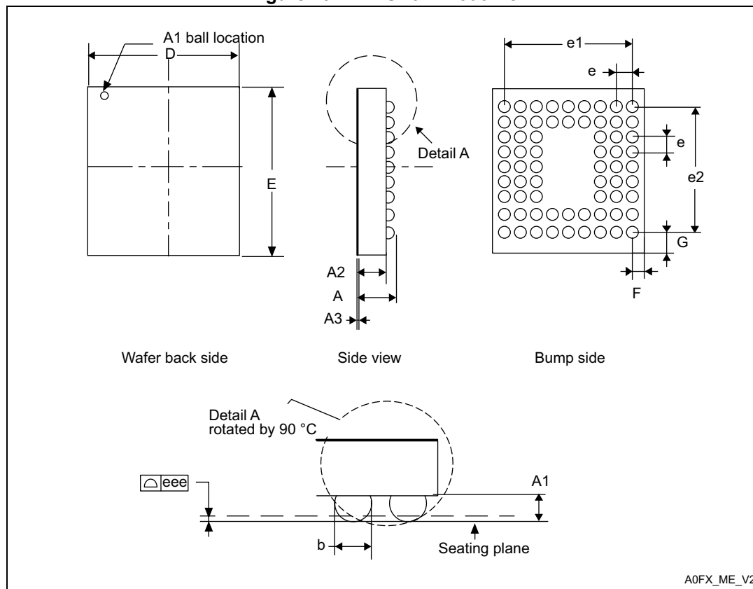
Figure 79. WLCSP64+2 outline
