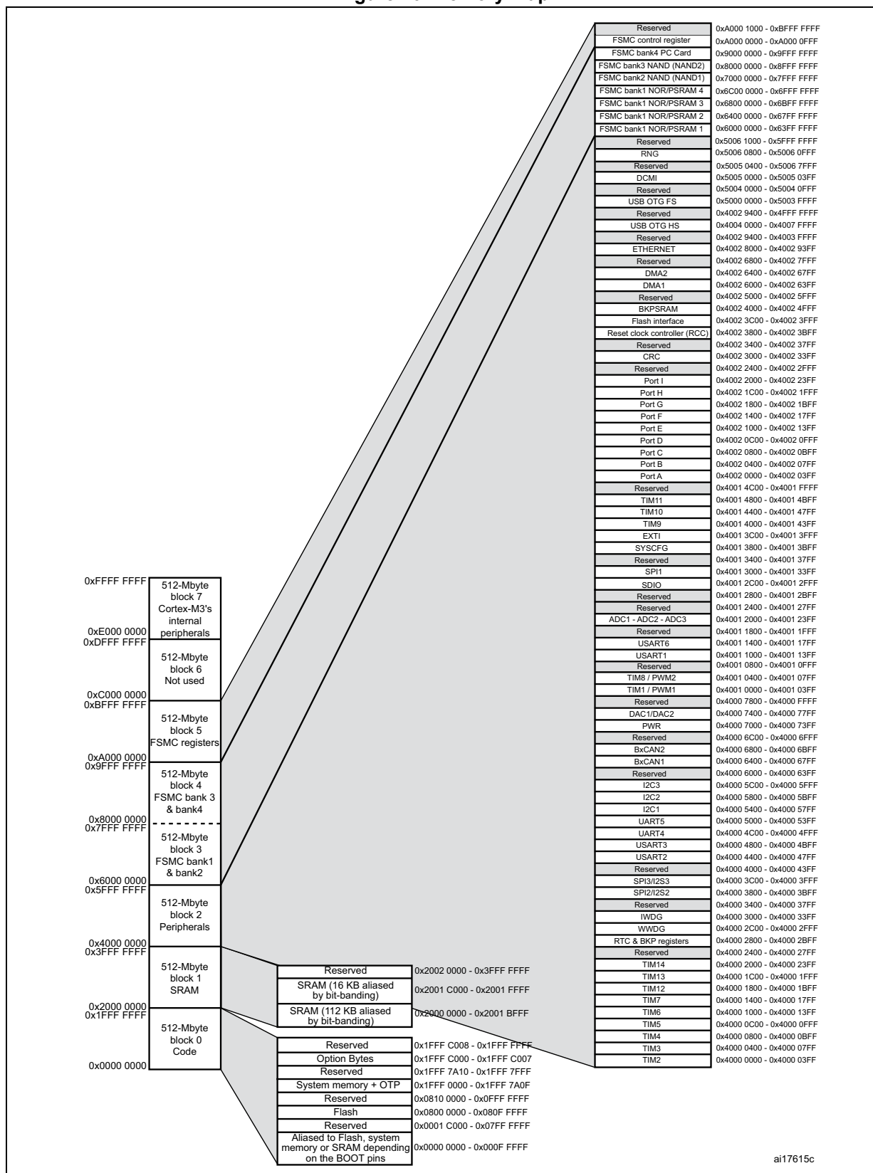
Figure 16. Memory map
