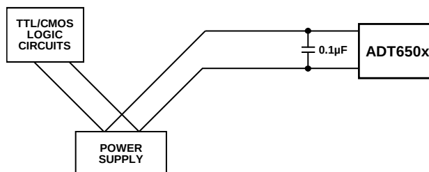
Figure 19. Separate Traces Used to Reduce Power Supply Noise
