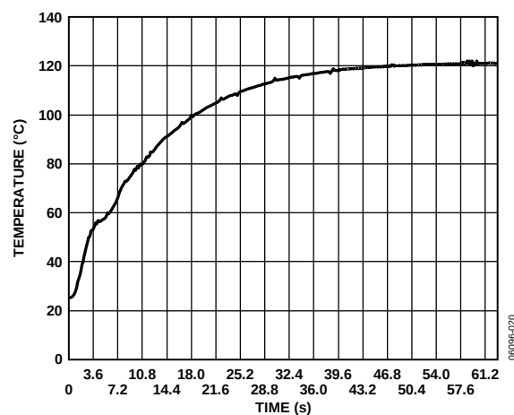
Figure 10. Thermal Step Response in Still Air
