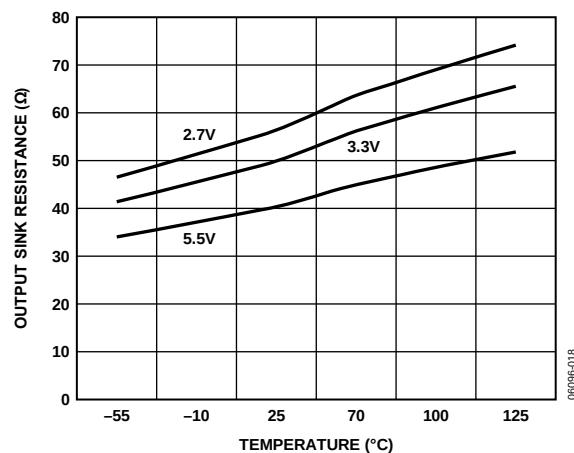
Figure 8. Output Sink Resistance vs. Temperature
