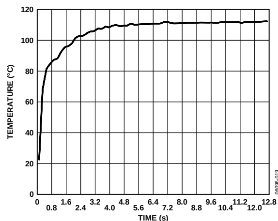
Figure 9. Thermal Step Response in Perfluorinated Fluid
