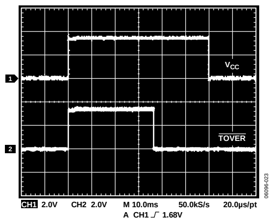
Figure 13. ADT6501 Start-Up Delay
