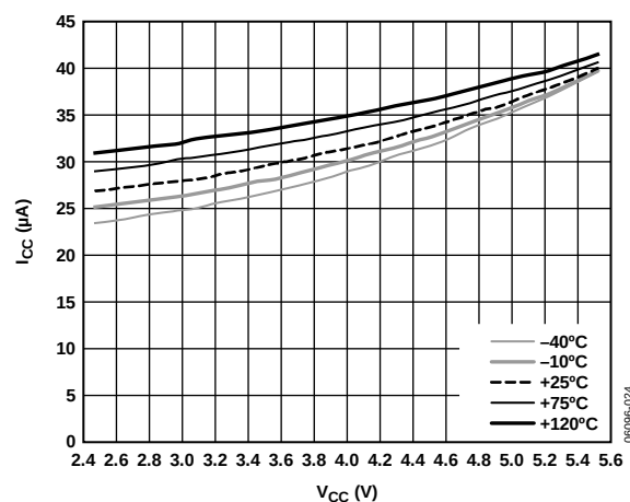
Figure 14. Operating Supply Current vs. Voltage Over Temperature
