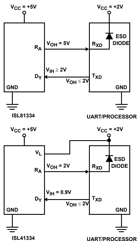
FIGURE 20. USING V I PIN TO ADJUST LOGIC LEVELS
