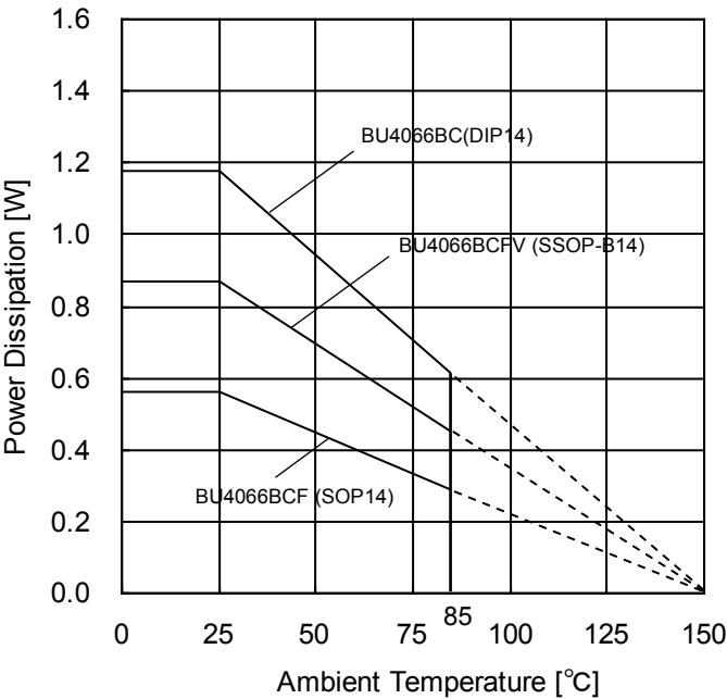
Figure 19. Derating Curve
