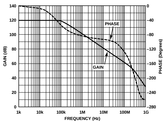
Figure 10. Transimpedance Gain and Phase vs. Frequency
