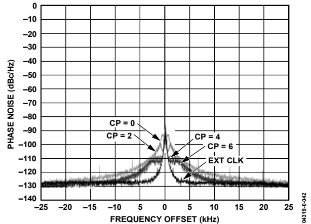
Figure 43. CLK Phase Noise vs. I_{BIAS} Setting (CKO); IF = 73.35 \text{ MHz} , IF = 71.1 \text{ MHz} , IFIN = -31 \text{ dBm} , f_{CLK} = 18 \text{ MHz} , f_{REF} = 16.8 \text{ MHz} ; CLK SYN Settings: CKO \text{ Bias} = 3 , CKR = 56 , and CKN = 60 with f_{REF} = 300 \text{ kHz}
