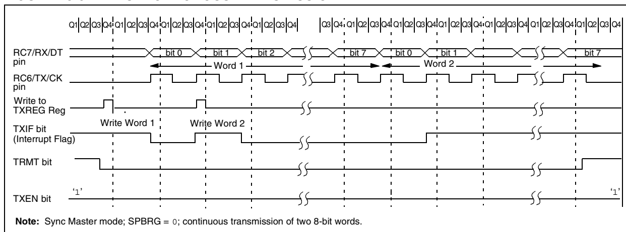
FIGURE 18-6: SYNCHRONOUS TRANSMISSION
