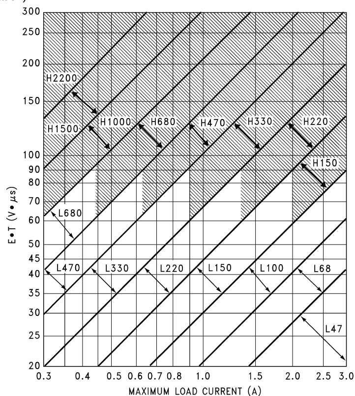
Figure 27. LM2576(HV)-ADJ
