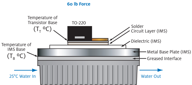
Water-cooled Heatsink
