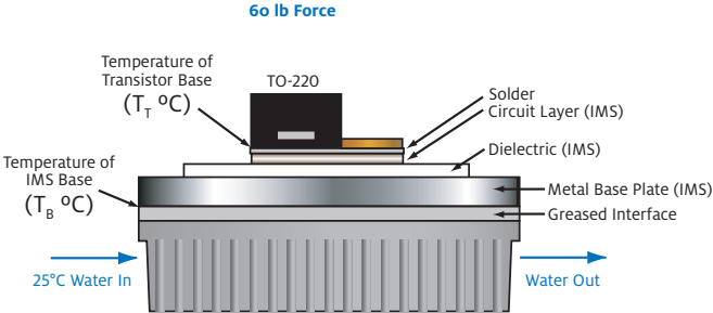
Water-cooled Heatsink
