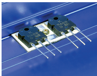
THERMAL CLAD measured junction temperature 5W= T_j 35°C
