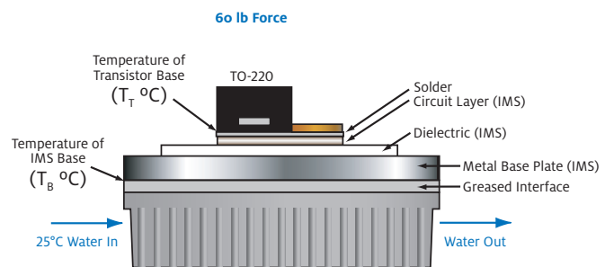
Water-cooled Heatsink
