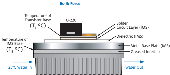
Water-cooled Heatsink
