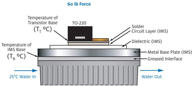
Water-cooled Heatsink
