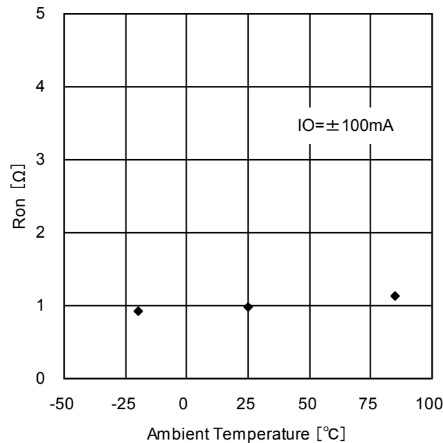
Figure 10. Output ON-Resistance Temperature Dependency (5ch,6ch driver block)
