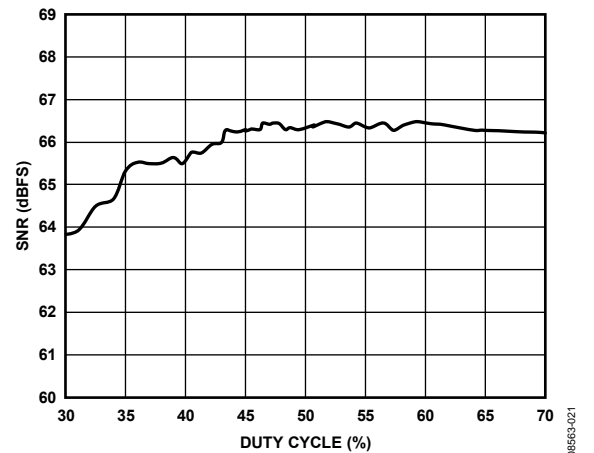
Figure 21. SNR vs. Duty Cycle with f_{IN} = 10.3 MHz
