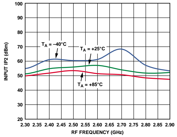
Figure 40. Input IP2 vs. RF Frequency at 3.3 V
