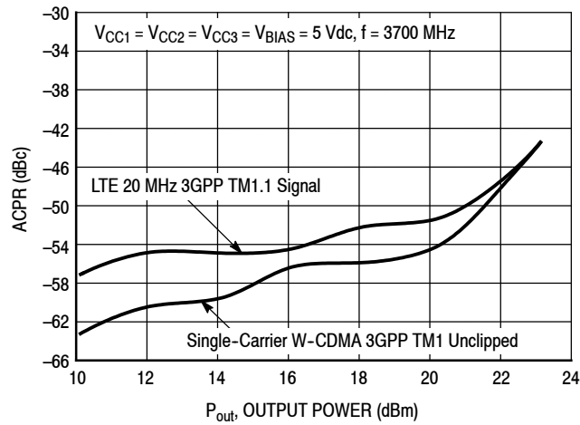
Figure 39. ACPR versus Output Power
