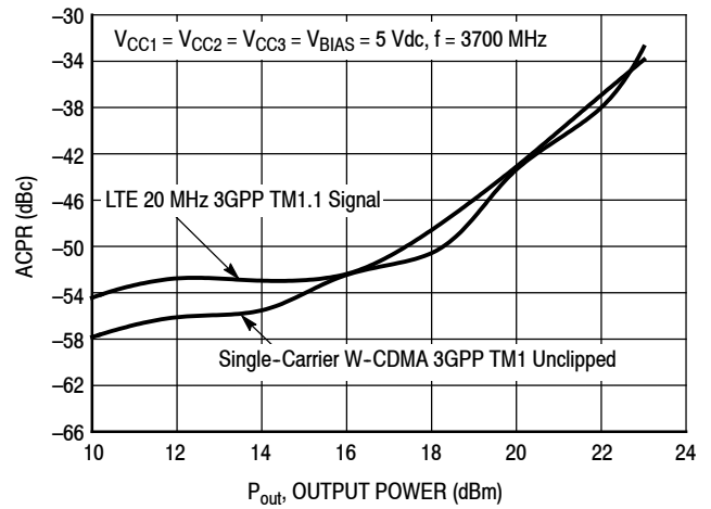
Figure 40. ACPR versus Output Power
