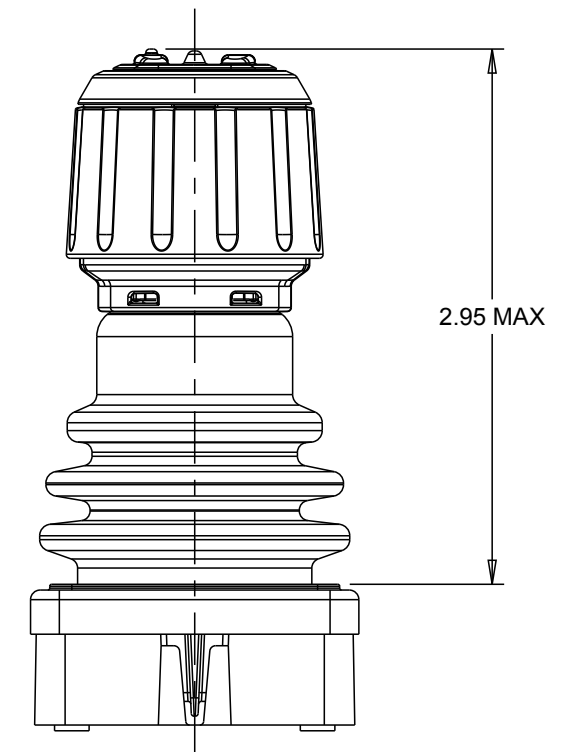
Z AXIS WITH PUSHBUTTONS
