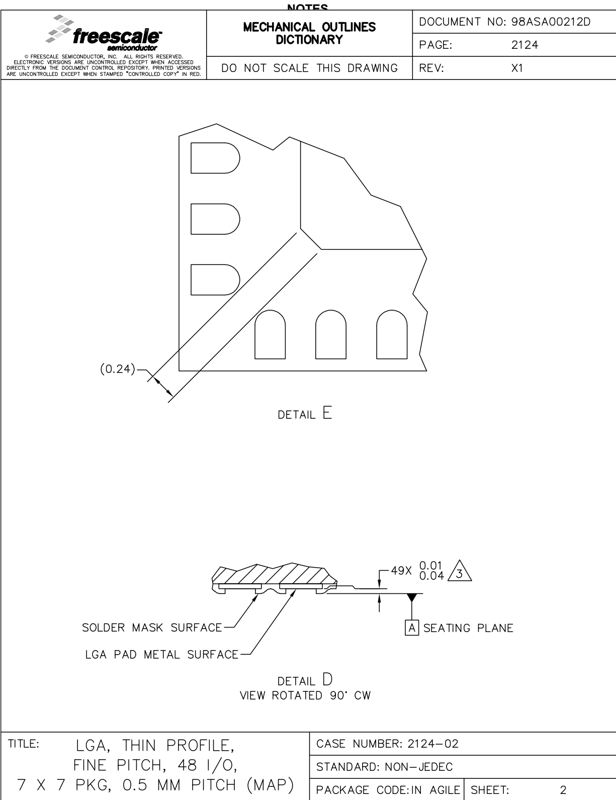
Figure 12. Mechanical Diagram (2 of 2)
