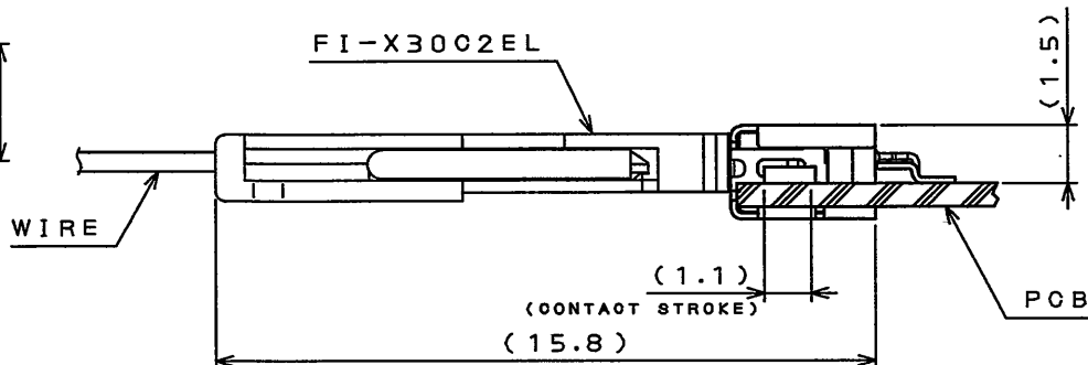
MATED CONDITION (REF.) 嵌合状態図 (参考)
