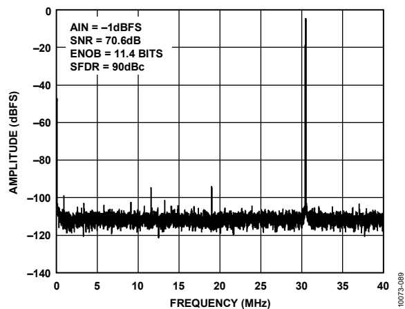
Figure 11. Single-Tone 16k FFT with f_{IN} = 30.5 \text{ MHz} , f_{SAMPLE} = 80 \text{ MSPS}
