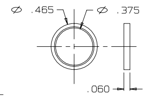
RING, STRAIN RELIEF TJSS-106-6
