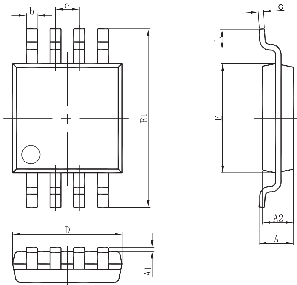
MSOP-8
