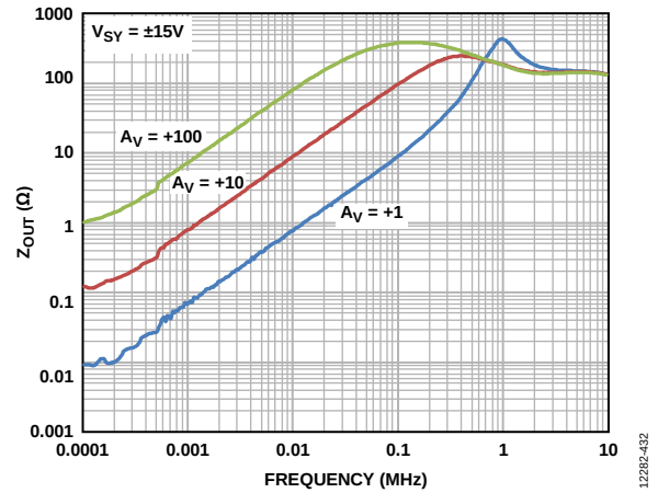
Figure 48. Output Impedance ( Z_{OUT} ) vs. Frequency, V_{SY} = \pm 15\text{ V}
