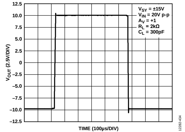
Figure 49. Large Signal Transient Response, V_{SY} = \pm 15\text{ V}
