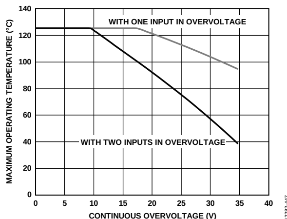
Figure 93. Maximum Operating Temperature vs. Continuous Overvoltage for One Input and Two Inputs ( \theta_{JA} = 150^\circ\text{C/W} )
