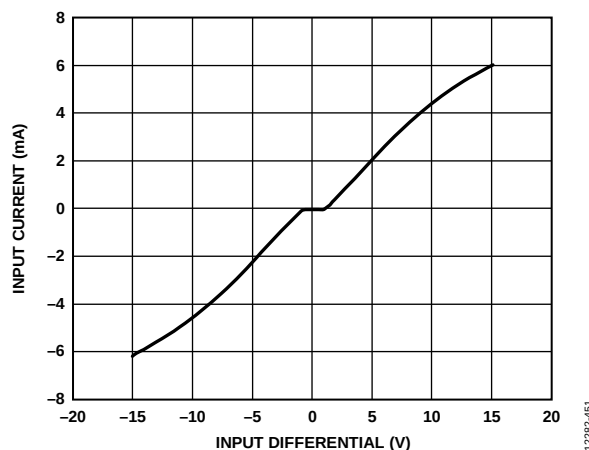
Figure 94. Input Current vs. Input Differential with \pm 15 V Supplies
