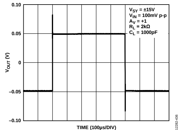
Figure 50. Small Signal Transient Response, V_{SY} = \pm 15\text{ V}
