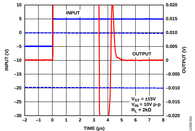
Figure 62. Positive Settling Time to 0.1%, V_{SY} = \pm 15\text{ V}
