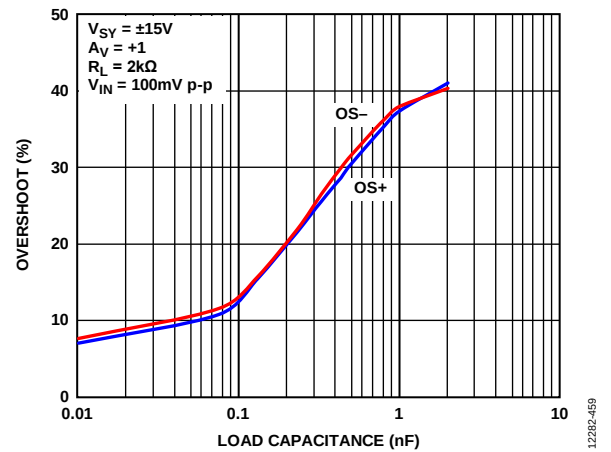
Figure 61. Small Signal Overshoot vs. Load Capacitance, V_{SY} = \pm 15\text{ V}
