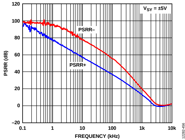
Figure 57. Power Supply Rejection Ratio (PSRR) vs. Frequency, V_{SY} = \pm 5\text{ V}
