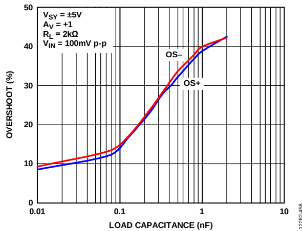
Figure 58. Small Signal Overshoot vs. Load Capacitance, V_{SY} = \pm 5\text{ V}
