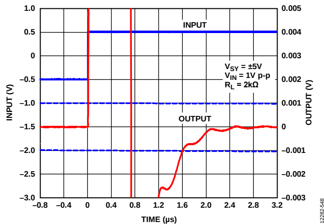
Figure 59. Positive Settling Time to 0.1%, V_{SY} = \pm 5\text{ V}
