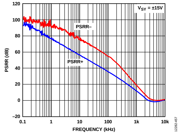
Figure 60. Power Supply Rejection Ratio (PSRR) vs. Frequency, V_{SY} = \pm 15\text{ V}
