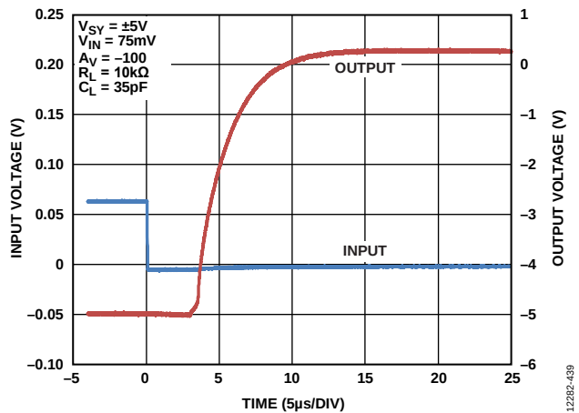
Figure 52. Negative Overload Recovery, V_{SV} = \pm 5 V
