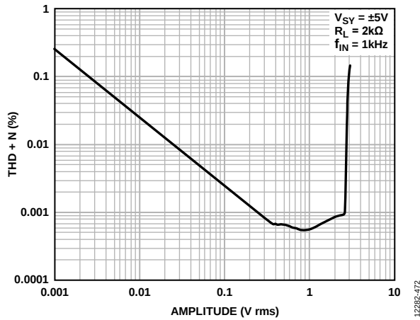
Figure 69. THD + N vs. Amplitude, V_{SY} = \pm 5\text{ V}
