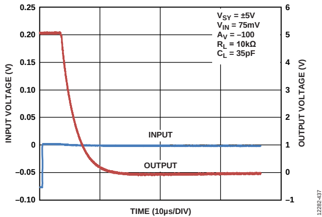
Figure 51. Positive Overload Recovery, V_{SV} = \pm 5 V
