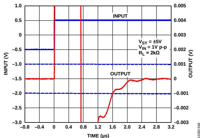
Figure 59. Positive Settling Time to 0.1%, V_{SV} = \pm 5V
