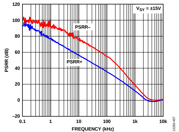
Figure 60. Power Supply Rejection Ratio (PSRR) vs. Frequency, V_{SV} = \pm 15V
