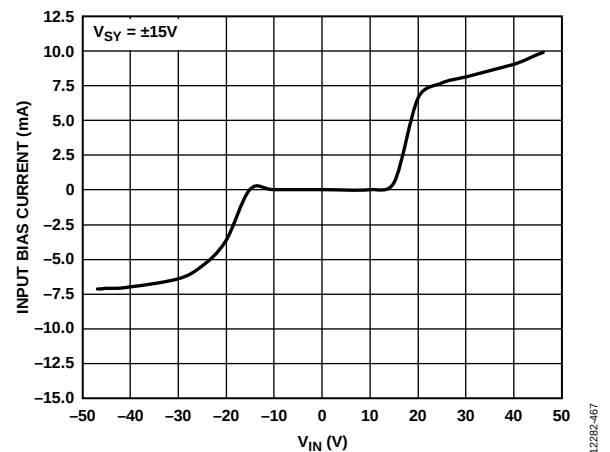
Figure 74. Input Bias Current vs. Input Voltage ( V_{IN} ) Including Input Overvoltage Range (Beyond V_{SY} = \pm 15\text{ V} )
