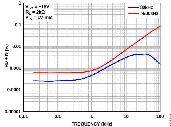
Figure 68. THD + N vs. Frequency, V_{SV} = \pm 15\text{ V}
