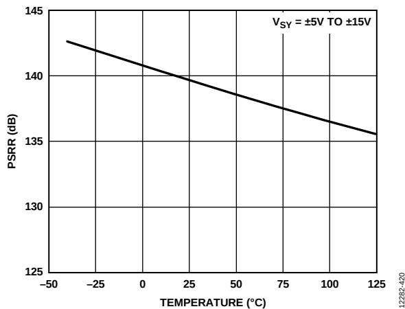
Figure 53. Power Supply Rejection Ratio (PSRR) vs. Temperature, V_{SV} = \pm 5 V to \pm 15 V
