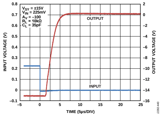
Figure 55. Negative Overload Recovery, V_{SV} = \pm 15 V
