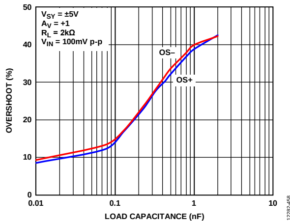
Figure 58. Small Signal Overshoot vs. Load Capacitance, V_{SV} = \pm 5V
