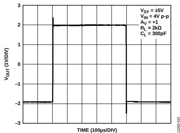
Figure 46. Large Signal Transient Response, V_{SY} = \pm 5\text{ V}
