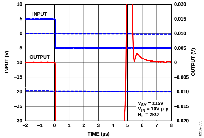
Figure 66. Negative Settling Time 0.1%, V_{SV} = \pm 15\text{ V}
