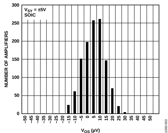
Figure 11. Input Offset Voltage ( V_{OS} ) Distribution, V_{SY} = \pm 5V , 14-Lead SOIC
