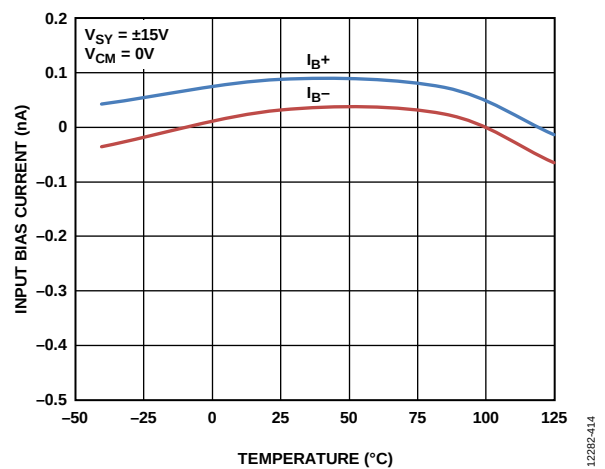
Figure 32. Input Bias Current ( I_B ) vs. Temperature, V_{SY} = \pm 15\text{ V}
