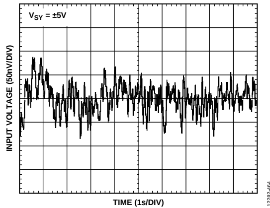
Figure 70. 0.1 Hz to 10 Hz Noise, V_{SY} = \pm 5\text{ V}
