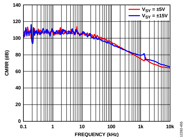
Figure 56. Common-Mode Rejection Ratio (CMRR) vs. Frequency, V_{SV} = \pm 5 V and V_{SV} = \pm 15 V
