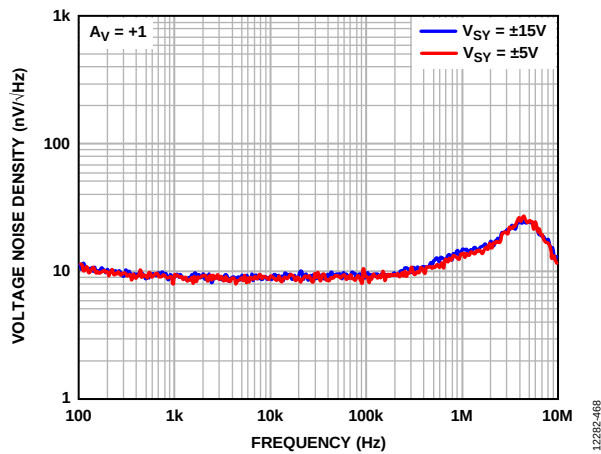
Figure 64. Voltage Noise Density vs. Frequency, V_{SV} = \pm 5\text{ V} and V_{SV} = \pm 15\text{ V}
