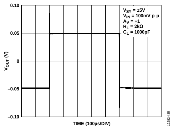
Figure 47. Small Signal Transient Response, V_{SY} = \pm 5\text{ V}
