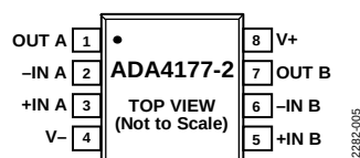
Figure 6. 8-Lead SOIC Pin Configuration, ADA4177-2
