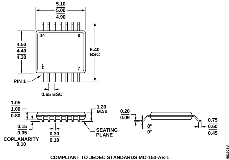
Figure 99. 14-Lead Thin Shrink Small Outline Package [TSSOP] (RU-14)
