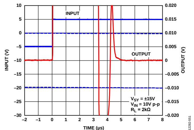
Figure 62. Positive Settling Time to 0.1%, V_{SV} = \pm 15V
