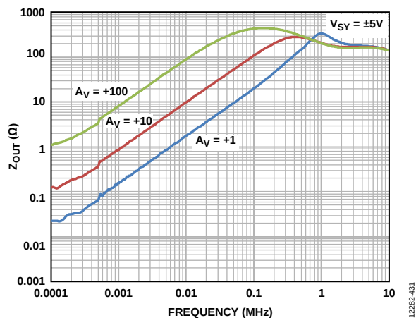
Figure 45. Output Impedance ( Z_{OUT} ) vs. Frequency, V_{SY} = \pm 5\text{ V}
