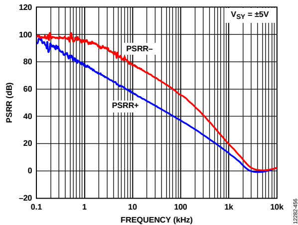
Figure 57. Power Supply Rejection Ratio (PSRR) vs. Frequency, V_{SV} = \pm 5V
