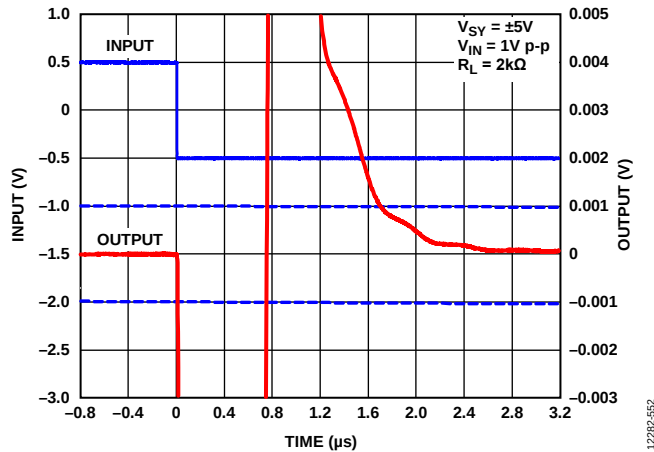
Figure 63. Negative Settling Time to 0.1%, V_{SV} = \pm 5\text{ V}
