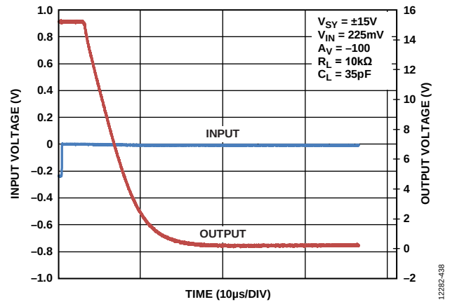
Figure 54. Positive Overload Recovery, V_{SV} = \pm 15 V
