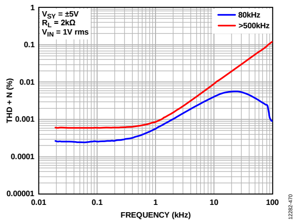
Figure 65. THD + N vs. Frequency, V_{SV} = \pm 5\text{ V}
