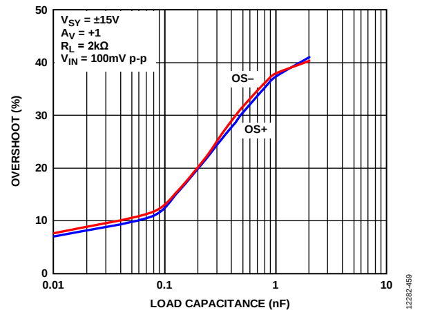
Figure 61. Small Signal Overshoot vs. Load Capacitance, V_{SV} = \pm 15V
