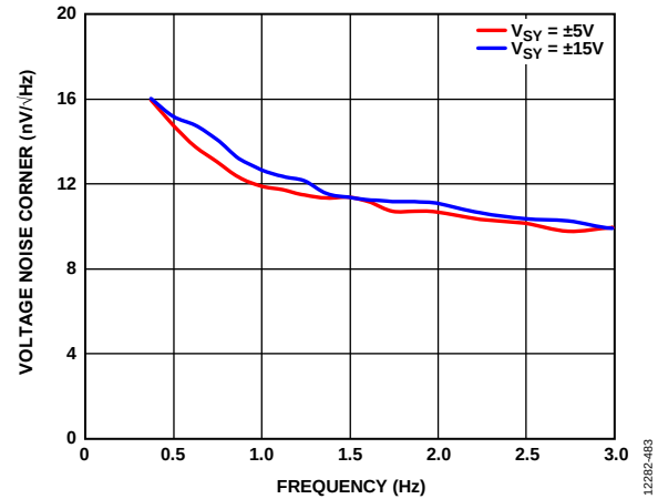
Figure 67. Voltage Noise Corner vs. Frequency, V_{SV} = \pm 5\text{ V} and V_{SV} = \pm 15\text{ V}
