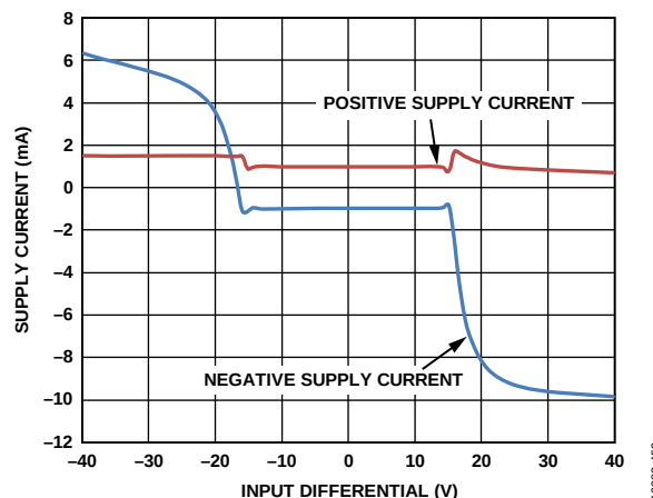
Figure 91. Supply Current vs. Input Differential, Circuit Configured at Unity Gain with V_+ = +15 V and V_- = -15 V
