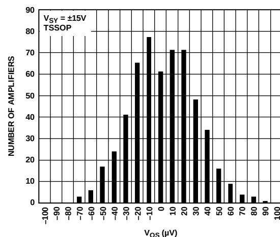
Figure 18. Input Offset Voltage ( V_{OS} ) Distribution, V_{SY} = \pm 15V , 14-Lead TSSOP
