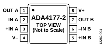
Figure 5. 8-Lead MSOP Pin Configuration, ADA4177-2
