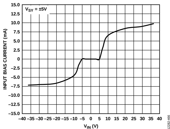
Figure 71. Input Bias Current vs. Input Voltage ( V_{IN} ) Including Input Overvoltage Range (Beyond V_{SY} = \pm 5\text{ V} )
