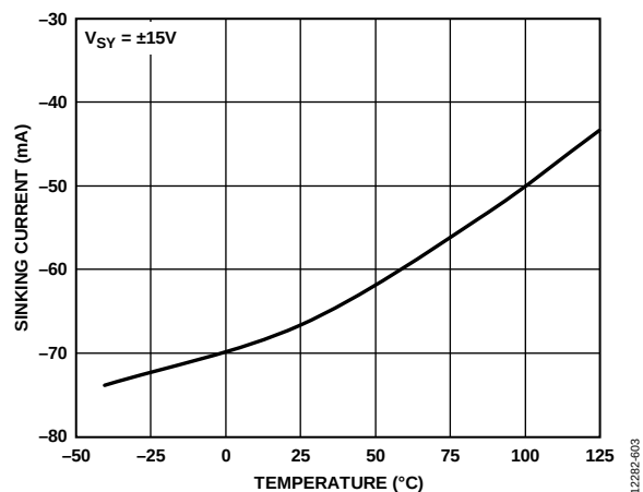
Figure 83. Output Short-Circuit Sinking Current vs. Temperature, V_{SY} = \pm 15V
