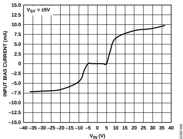
Figure 71. Input Bias Current vs. Input Voltage ( V_{IN} ) Including Input Overvoltage Range (Beyond V_{SV} = \pm 5\text{ V} )
