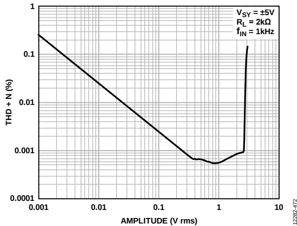
Figure 69. THD + N vs. Amplitude, V_{SV} = \pm 5\text{ V}
