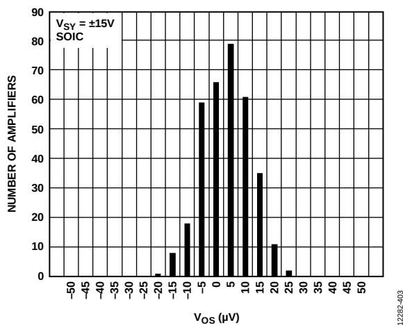
Figure 12. Input Offset Voltage ( V_{OS} ) Distribution, V_{SY} = \pm 15\text{ V} , 8-Lead SOIC
