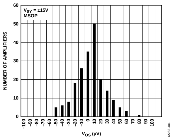
Figure 13. Input Offset Voltage ( V_{OS} ) Distribution, V_{SY} = \pm 15\text{ V} , 8-Lead MSOP
