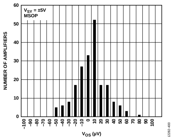
Figure 10. Input Offset Voltage ( V_{OS} ) Distribution, V_{SY} = \pm 5\text{ V} , 8-Lead MSOP
