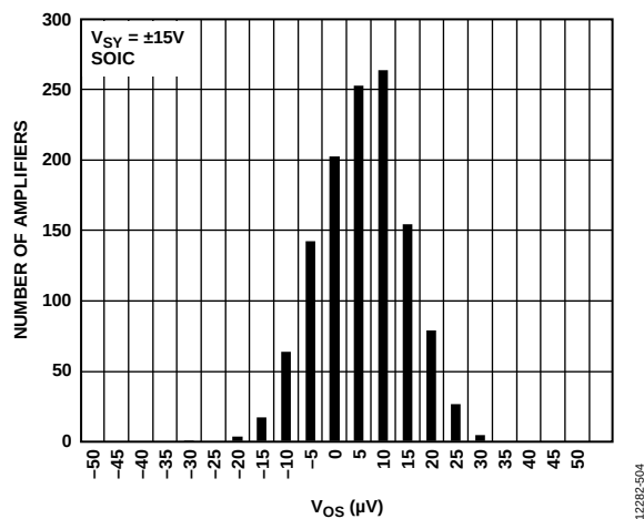
Figure 14. Input Offset Voltage ( V_{OS} ) Distribution, V_{SY} = \pm 15\text{ V} , 14-Lead SOIC
