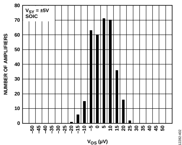
Figure 9. Input Offset Voltage ( V_{OS} ) Distribution, V_{SY} = \pm 5\text{ V} , 8-Lead SOIC
