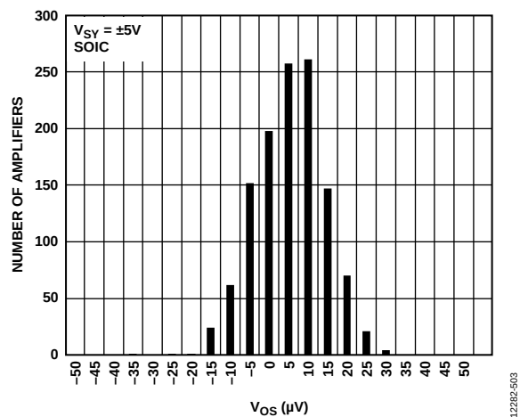
Figure 11. Input Offset Voltage ( V_{OS} ) Distribution, V_{SY} = \pm 5\text{ V} , 14-Lead SOIC
