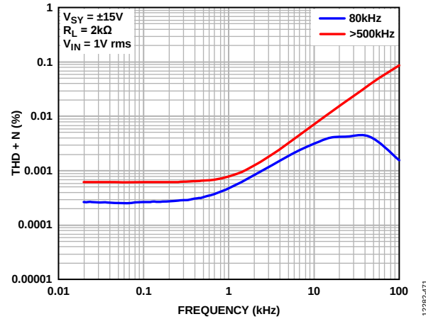
Figure 68. THD + N vs. Frequency, V_{SV} = \pm 15V
