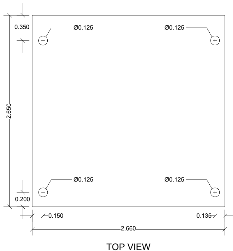
Figure 2.2 EVB9512 Mechanicals
