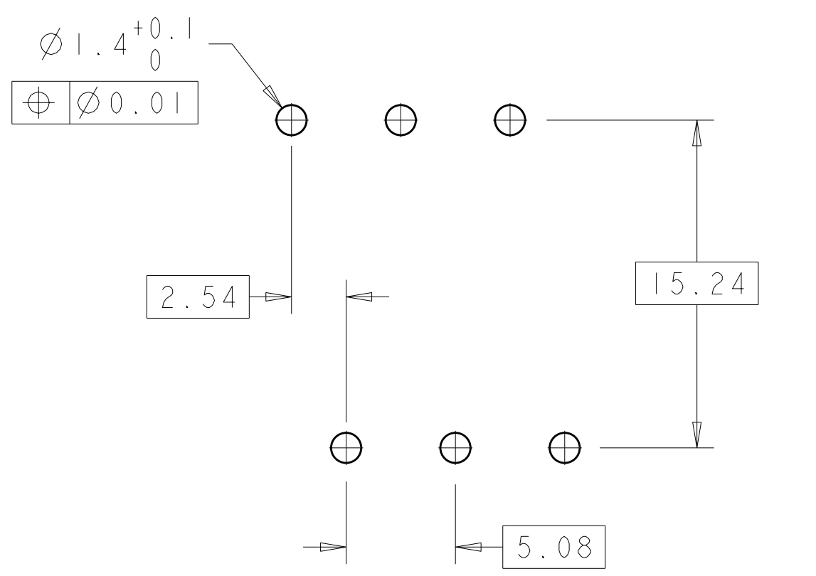
RECOMMENDED PC BOARD LAYOUT ACCEPTS 1.6 - 2.4 mm PC BOARD THICKNESS
