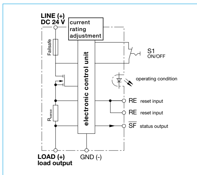
Schematic diagram ESX10-S127 (example)
