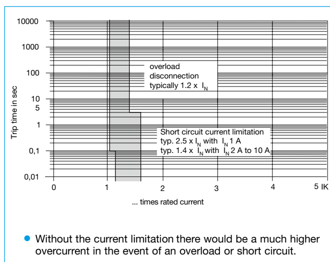
Time/current characteristic curve ( T_{amb} = 25\text{ °C} , U_B = \text{DC } 24\text{ V} )
